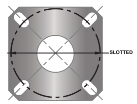
AL-4 TEMPLATE 10.00 X 10.00 X 0.75 ANCHOR PLATE 9.50" - 10.25" DIA. BOLT CIRCLE
