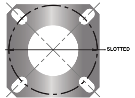
AL-5 TEMPLATE 11.00 X 11.00 X 1.00 ANCHOR PLATE 11.50\"/>
