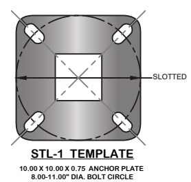
ANCHOR BOLT
