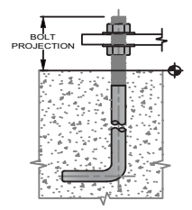
ANCHOR BOLT
