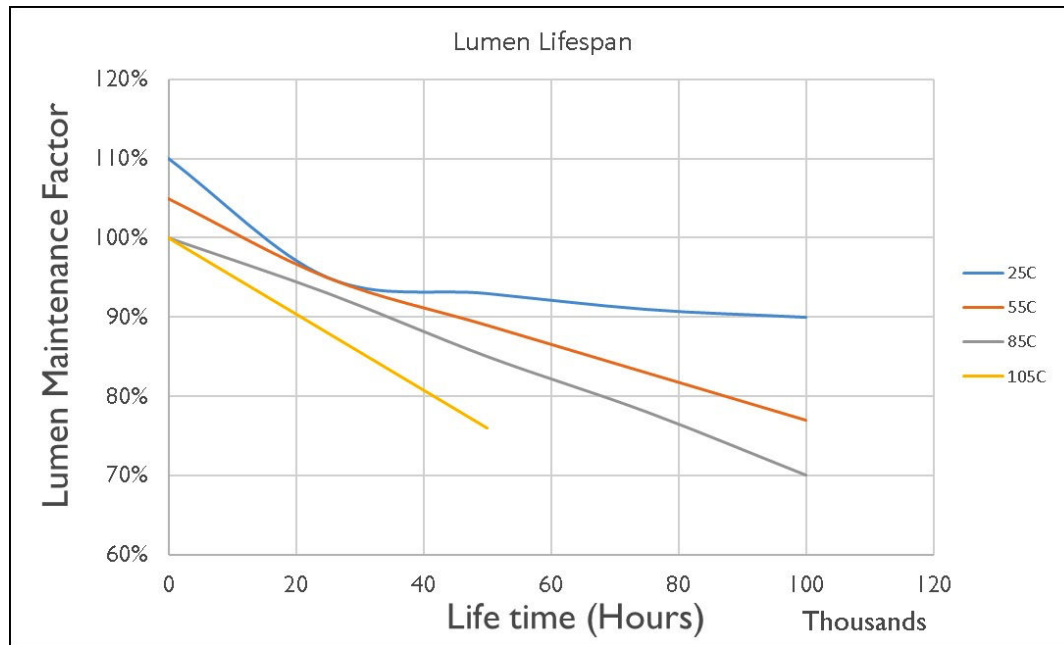
Lumen Maintenance Factors (B Drive)
