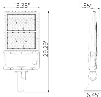
MSF-AR-00 200W-300W Slip Fitter
