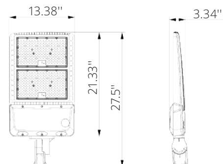
MYK-AR-00 200W-300W YM Bracket
