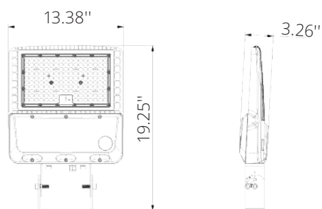
MTR-AR-00 60W-150W Trunnion Bracket
