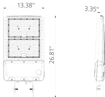
MYK-AR-00 200W-300W YM Bracket
