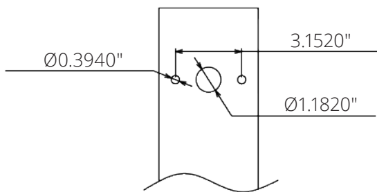
Trunnion Mount Pole drilling detail
