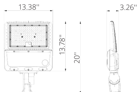
MYK-AR-00 60W-150W YM Bracket
