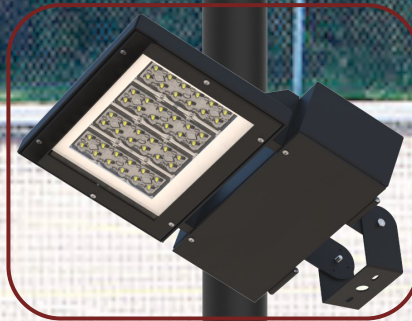
TRUNNION MOUNT
