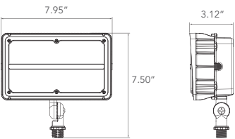
Knuckle Mount
