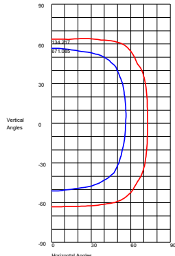
ISOCANDELA CURVES
