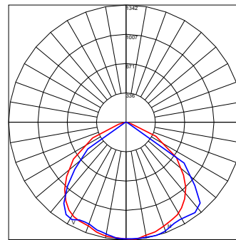
AXIAL CANDELA DISPLAY
