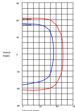
ISOCANDELA CURVES
