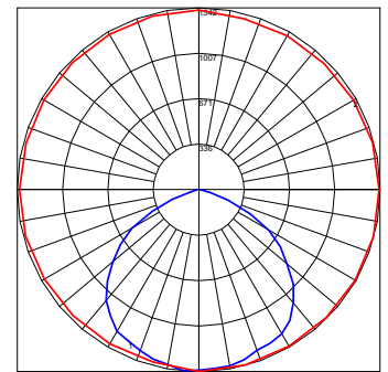
POLAR GRAPH
