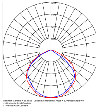
AXIAL CANDELA DISPLAY
