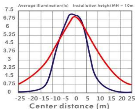
Average illumination curve
