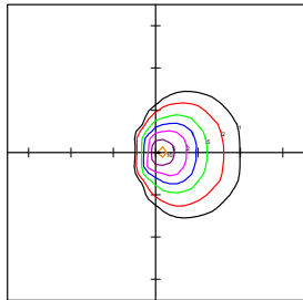
WPMP-24-50K@10' Replaces 60W-100W
