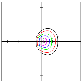
WPMP-12-50K@10' Replaces 60W-100W
