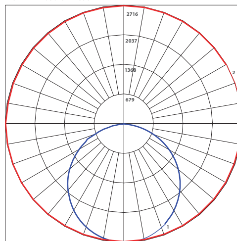
Polar Graph Neptun Light, Inc. LED-1LH24-080-UNV-850
