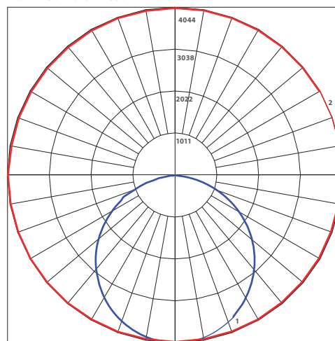
Polar Graph Neptun Light, Inc. LED-1LH36-120-UNV-850
