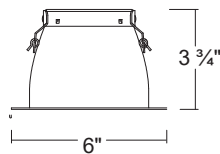
CVI4S-XX (4")
