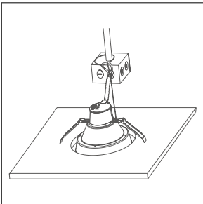
Ensure fixture is flush. Installation is complete
