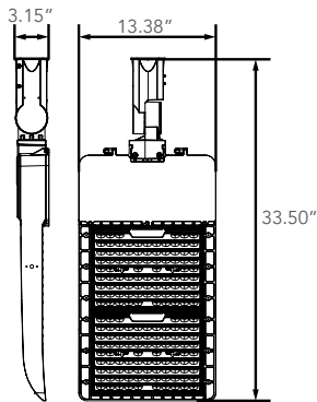
Slip Fitter
