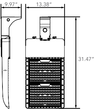
Pole Mount
