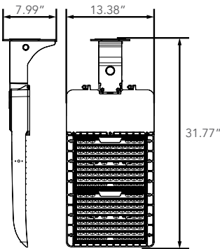
Wall Mount
