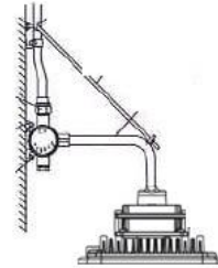
C. Wall Mount
