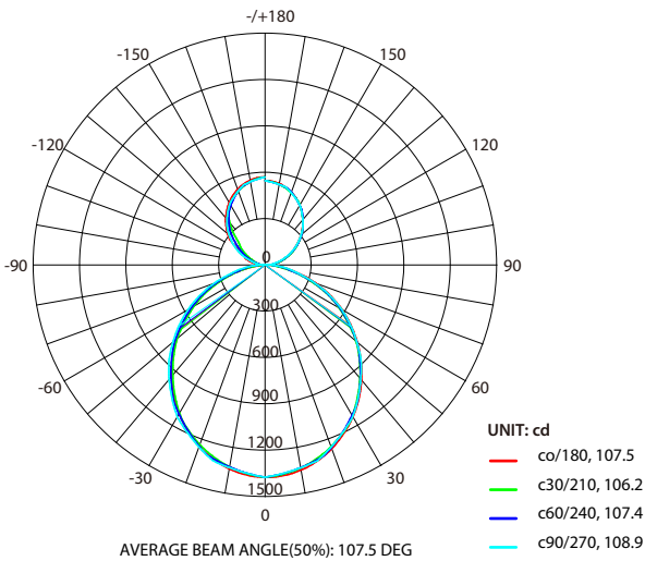
Polar Graph – 4’ Direct&Indirect Light 50W 4000K
